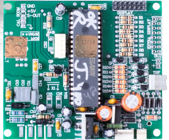
JEWELLERY PCB J400
