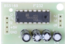
RS 232 PCB DATA TRANSFER
