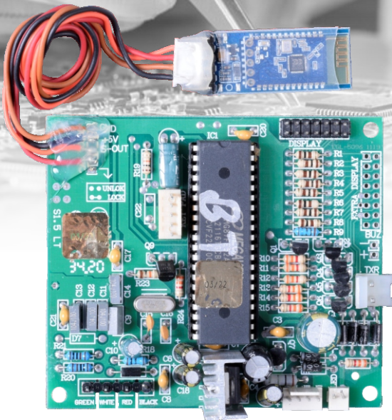
EGL BLUETOOTH PCB (Hc05) 6V RANGE 10 MTRS
