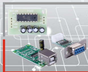
Rs232, SERIAL/TTL TO USB & TTL TO Rs232 CONVERTOR
