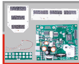
EGL PC 01 PRICE COMPUTING PIECE COUNTING, RTC, PRINTER
