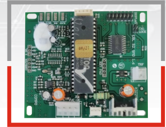
EGL S2 SMD (SINGLE PCB) 6V
